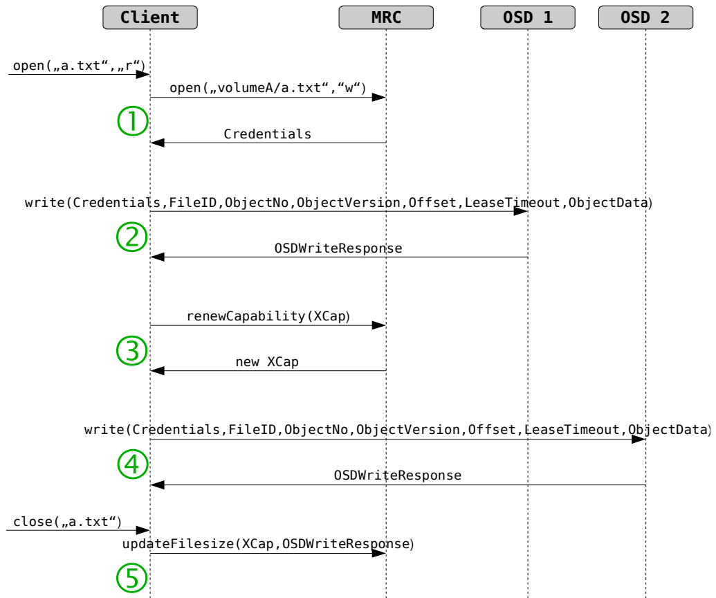
Figure 6.3: Writing a file
